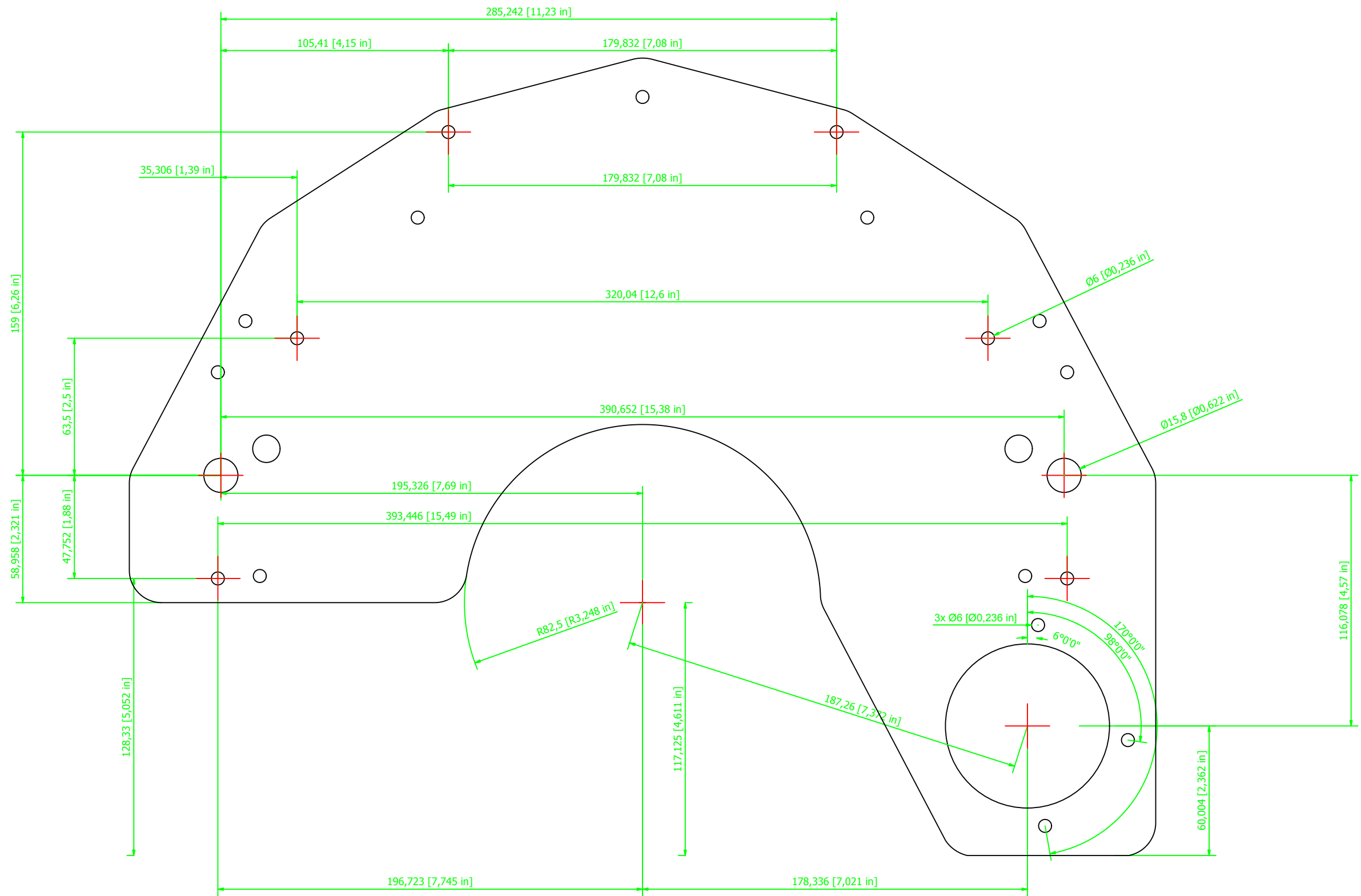
ADAPTOR PLATE LASER CUT FROM 6.5MM [0.25"] PLATE
