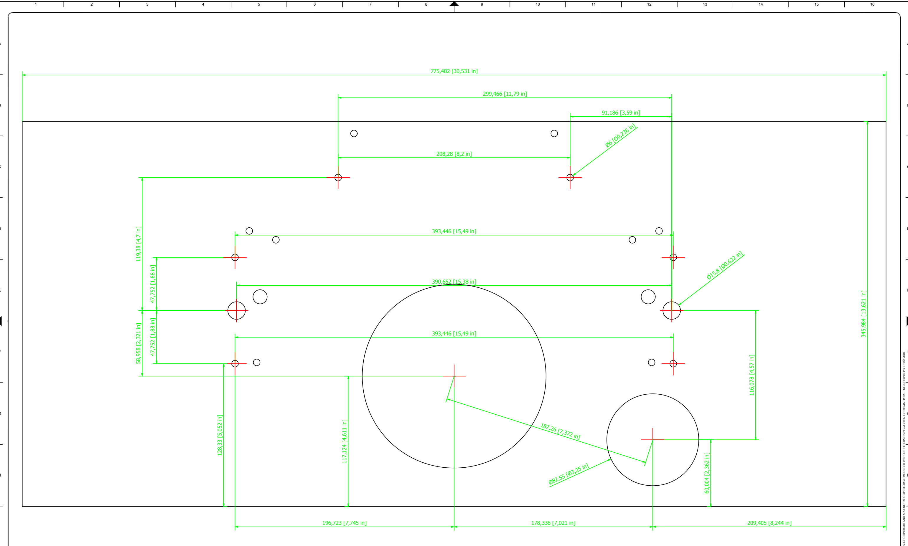
ADAPTOR PLATE LASER CUT FROM 6.5MM [0.25"] PLATE
