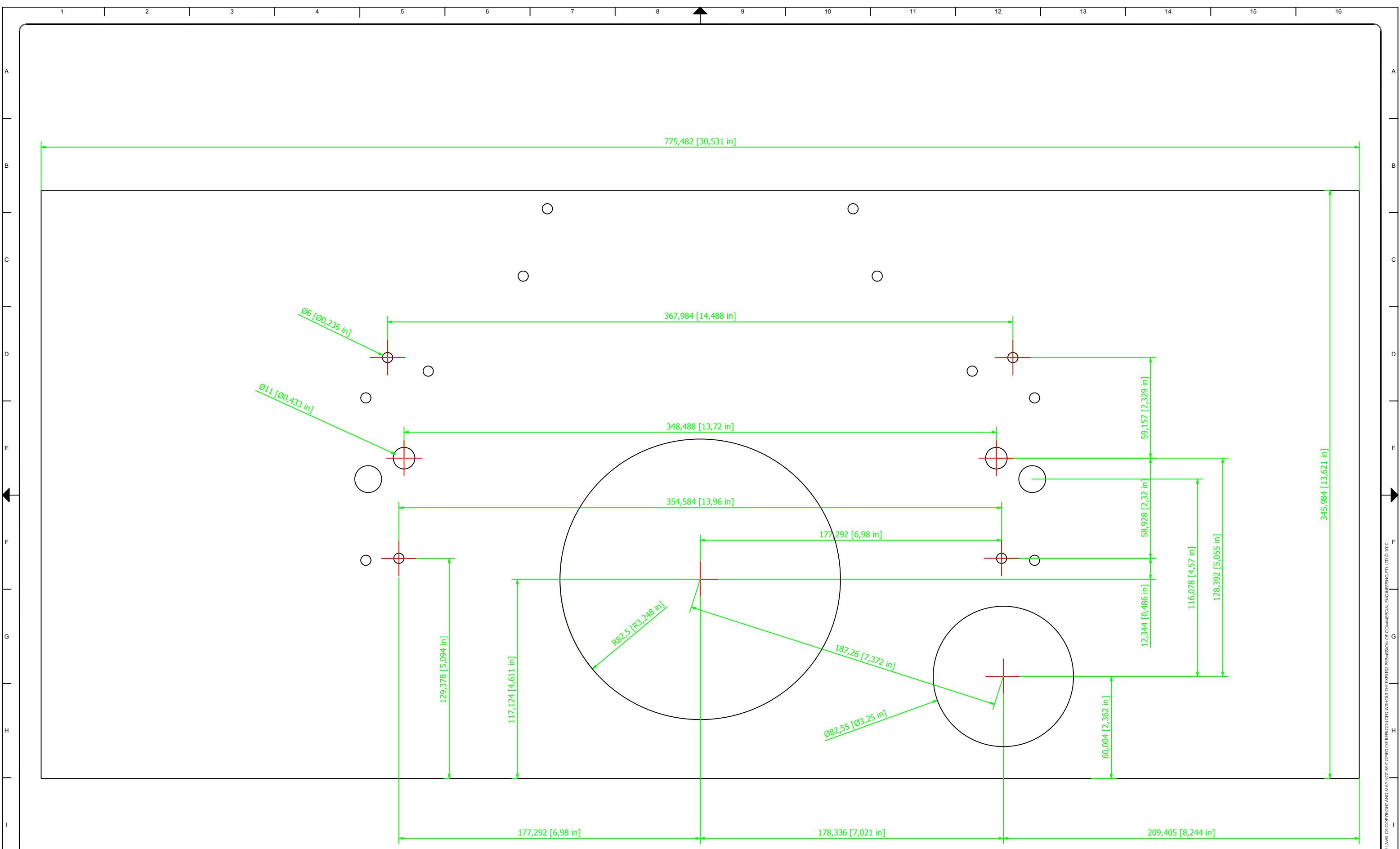
ADAPTOR PLATE LASER CUT FROM 6.5MM [0.25"] PLATE
